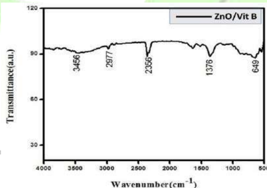
Fig.4: FTIR spectrum of ZnO/VB 1 /PVC NCs
