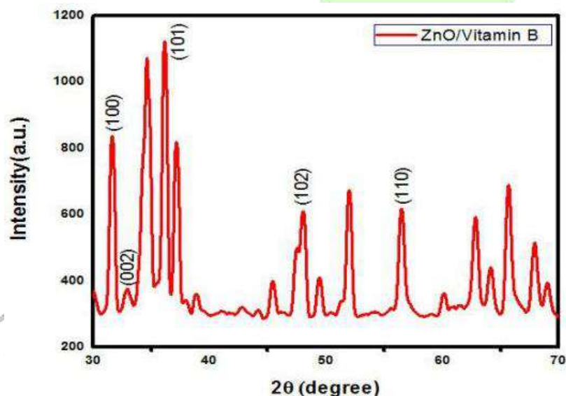
Fig.1: PXRD Pattern of ZnO/VB 1 NCs (2wt%)
