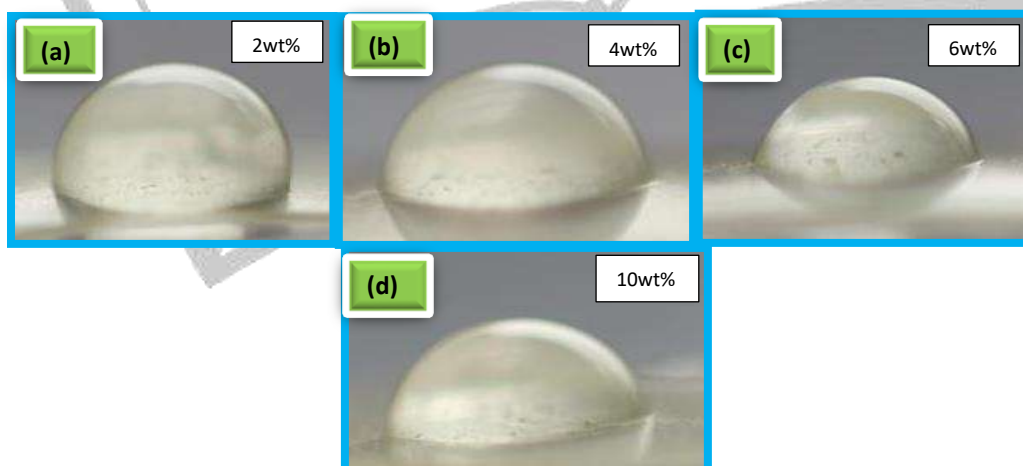
Fig.3: Contact angle measurements of ZnO/VB 1 NCs
