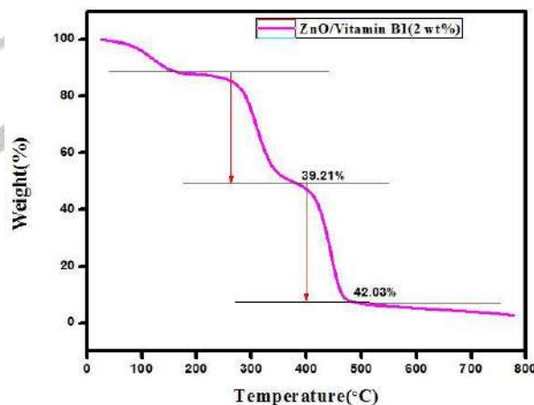
Fig.5: TGA Thermogram of ZnO/VB 1 /PVC NCs
